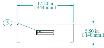
R.S. VIEW
